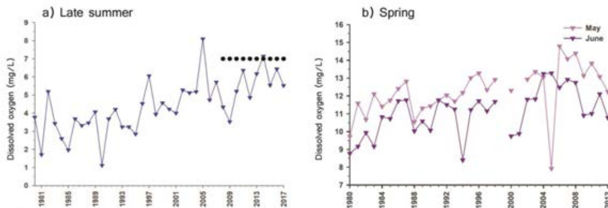
Figure 6-8 Long-term dissolved oxygen trends in Lake Simcoe in late summer and spring: (a) minimum late summer volume-weighted deep-water dissolved oxygen concentration between 1980 and 2017 (MECP, 2019), the dotted line denotes the LSPP target of 7 mg/L; (b) mean spring volume-weighted dissolved oxygen concentration (MOECC, 2015).
