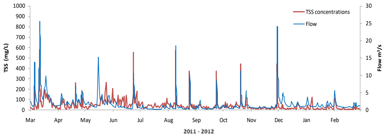
Figure 3-15 Average daily TSS concentrations at the East Holland River station (urban catchment).
