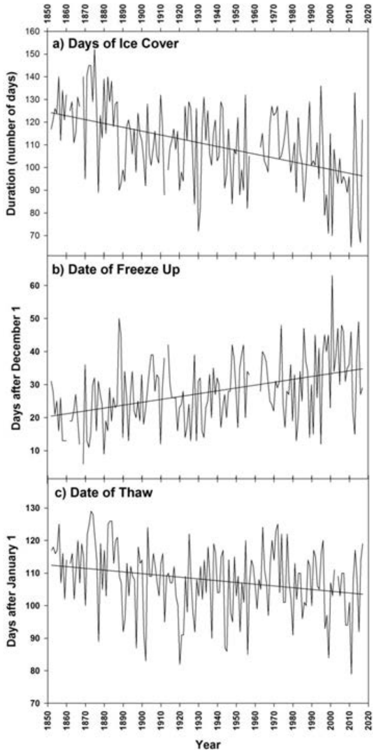
Figure 6-5 Long-term (1852-2017) ice cover trends for Kempfenfelt Bay: a) duration of ice cover; b) date of freeze-up as number of days after December 1; c) date of thaw as number of days after January 1. Solid line is linear regression trend line (data courtesy of Alex Mills, pers. comm.).
