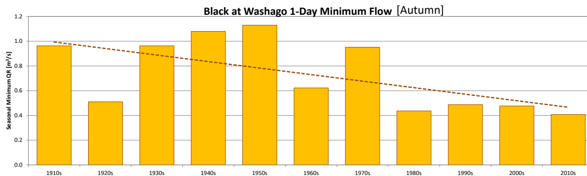
Figure 4-20 Single-day minimum flow in summer (a) and autumn (b) at the Black River - near Washago station (1915-2015) (Aspden, 2014).
