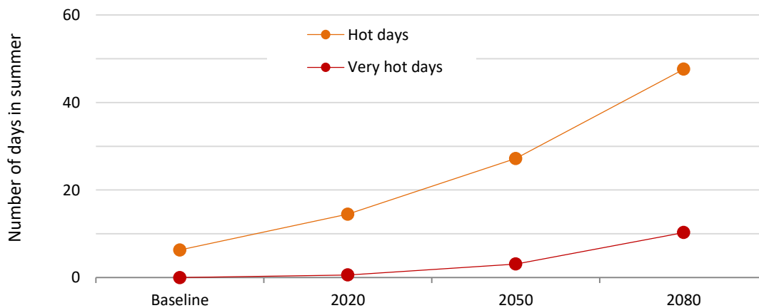
Figure 2-7 The average annual number of hot (> 30°C) and very hot (> 35°C) days in the summer (June, July and August) at Shanty Bay climate station based on the RCP8.5 climate scenario. Data source: Environment Canada (baseline) and Climate Change Hazards Information Portal (projection).
