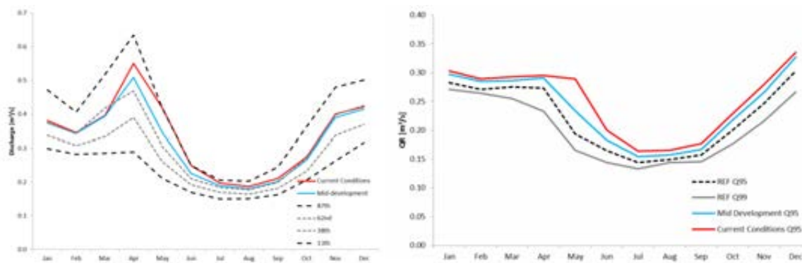
Figure 4-21 Modelled baseflow (left) and subsistence flows (right) for the Lovers Creek subwatershed.
