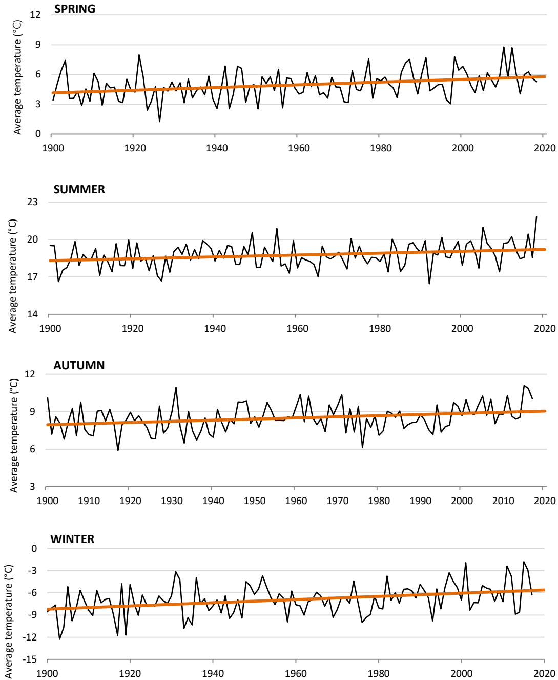
Figure 2-4 The observed temperatures averaged across 107 climate stations in the watershed presented seasonally between 1900 and 2017. The orange lines show the rate of warming in spring (0.013°C per year), summer (0.006°C per year), autumn (0.009°C per year), and winter (0.021°C per year). Trends are significant at p < 0.05 . Data source: Environment Canada daily timeseries averaged across 107 climate stations.
