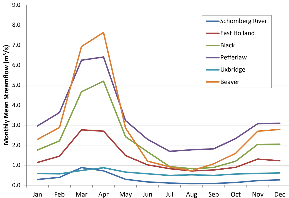
Figure 4-16 Monthly mean streamflow measurements at six gauged stations (1965-2018)
