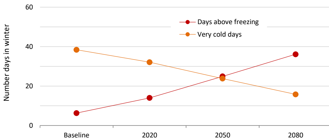
Figure 2-8 Projected annual average number of days above freezing (days with temperature greater than 0°C) and the number of very cold days (days with temperatures lower than -10°C) at Shanty Bay climate station in the RCP8.5 scenario. Data source: Environment Canada (baseline) and Climate Change Hazards Information Portal (projection).
