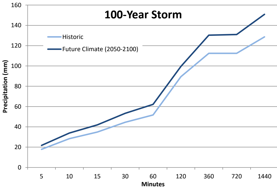
Figure 2-17 Intensity-duration-frequency (IDF) curves at the Barrie WPC ID:6110557 Station for the historic (1979-2007) and future (2050-2100) time periods under the RCP8.5 scenario. Data Source: Western University (2018).
